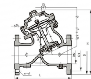
DIAPHRAGM TYPE
